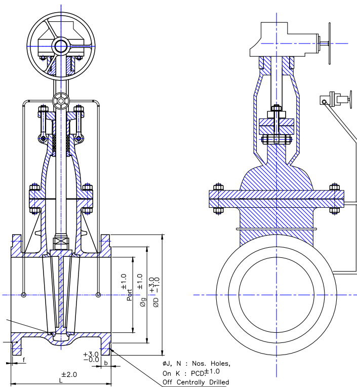
GATE VALVE WITH BY PASS ARRANGEMENT
